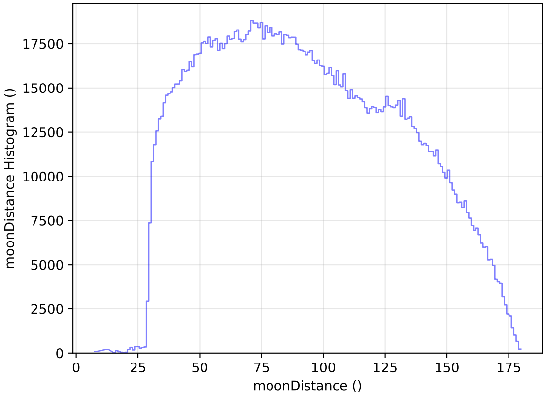
baseline_v3.2_10yrs WFD all bands: moonDistance Histogram
