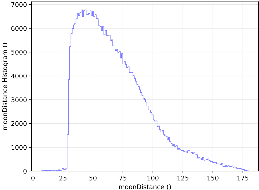
baseline_v3.2_10yrs All sky y band: moonDistance Histogram
