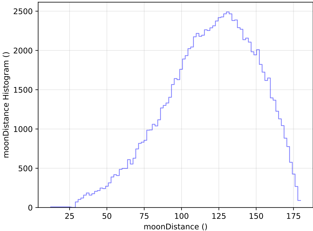
baseline_v3.2_10yrs All sky u band: moonDistance Histogram
