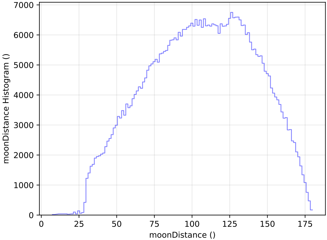
baseline_v3.2_10yrs All sky r band: moonDistance Histogram
