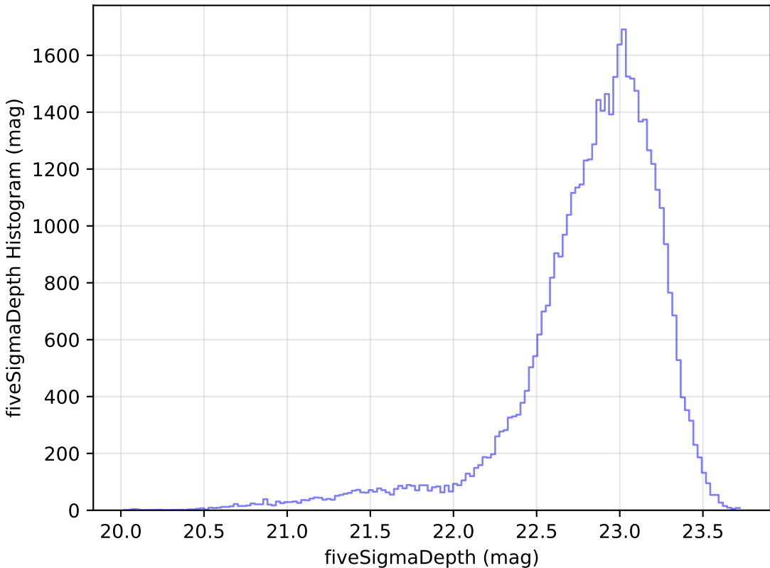
baseline_v3.2_10yrs Yr 1 z band: fiveSigmaDepth Histogram
