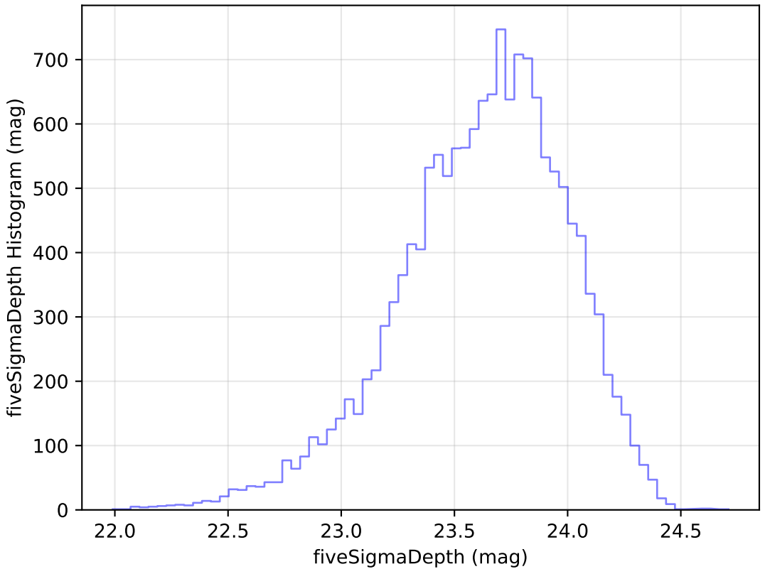
baseline_v3.2_10yrs Yr 1 u band: fiveSigmaDepth Histogram
