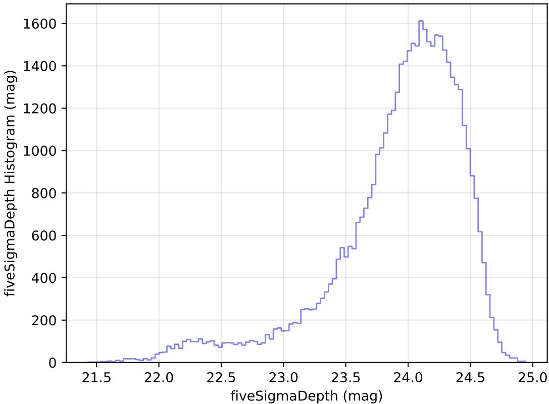
baseline_v3.2_10yrs Yr 1 r band: fiveSigmaDepth Histogram
