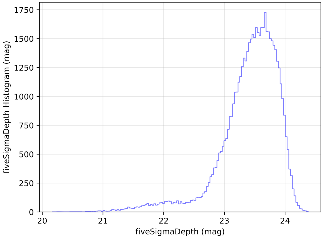
baseline_v3.2_10yrs Yr 1 i band: fiveSigmaDepth Histogram
