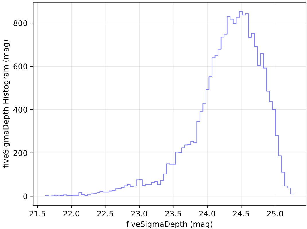
baseline_v3.2_10yrs Yr 1 g band: fiveSigmaDepth Histogram
