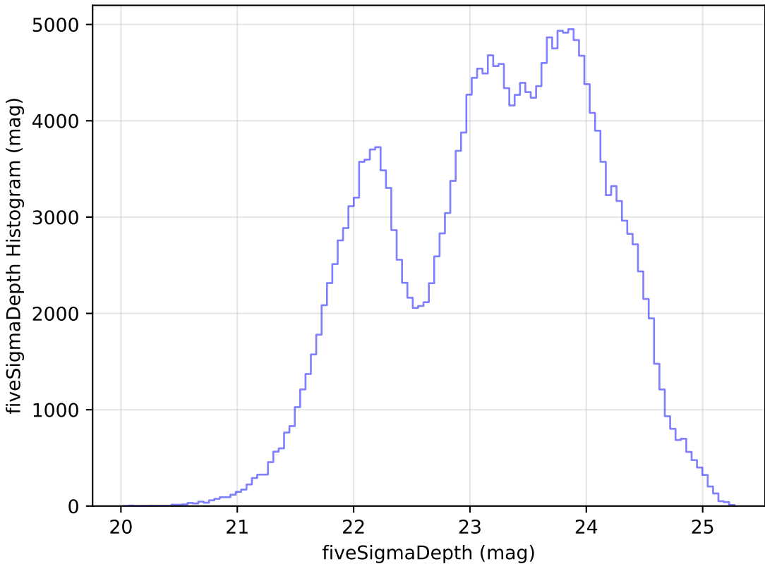
baseline_v3.2_10yrs Yr 1 all bands: fiveSigmaDepth Histogram
