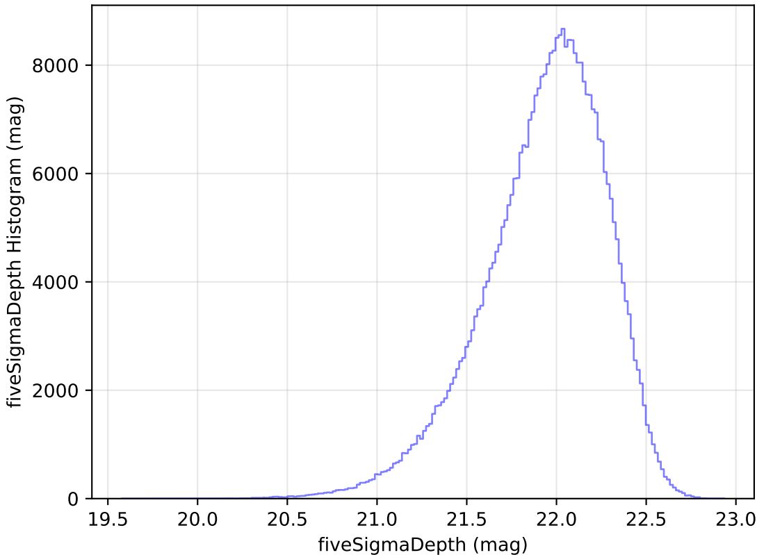
baseline_v3.2_10yrs WFD y band: fiveSigmaDepth Histogram
