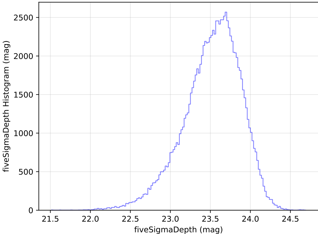
baseline_v3.2_10yrs WFD u band: fiveSigmaDepth Histogram
