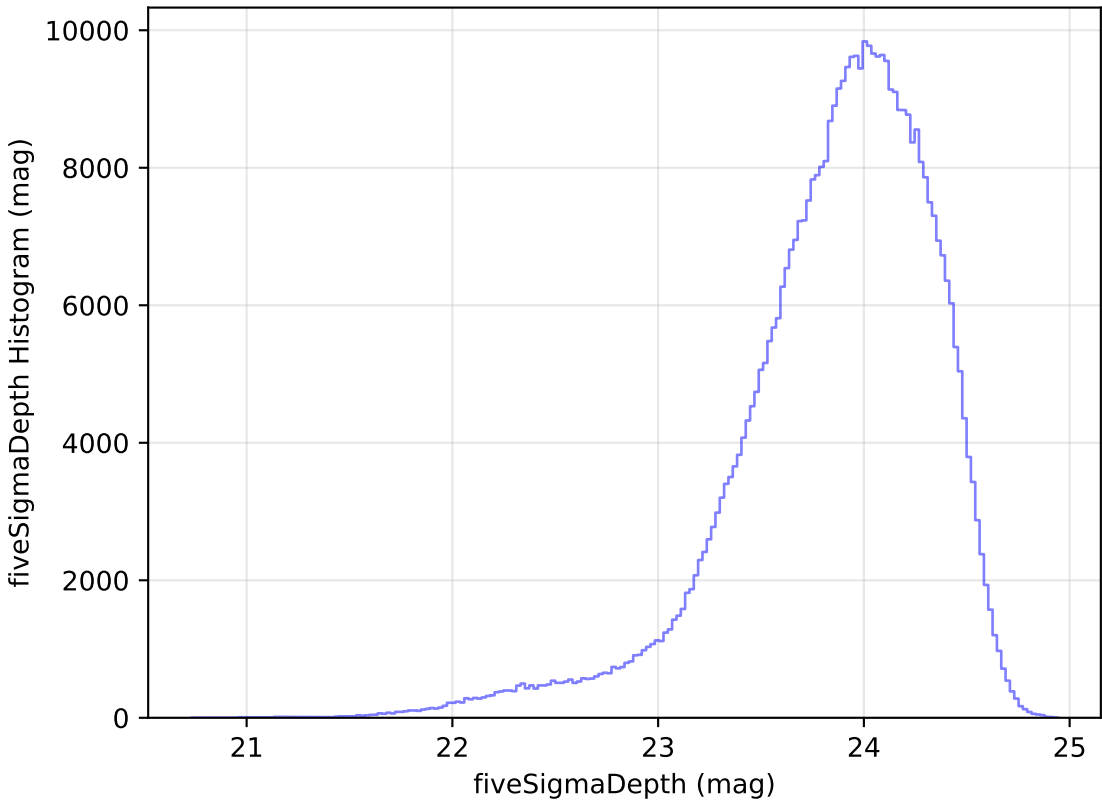
baseline_v3.2_10yrs WFD r band: fiveSigmaDepth Histogram
