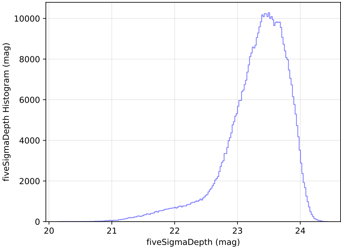
baseline_v3.2_10yrs WFD i band: fiveSigmaDepth Histogram
