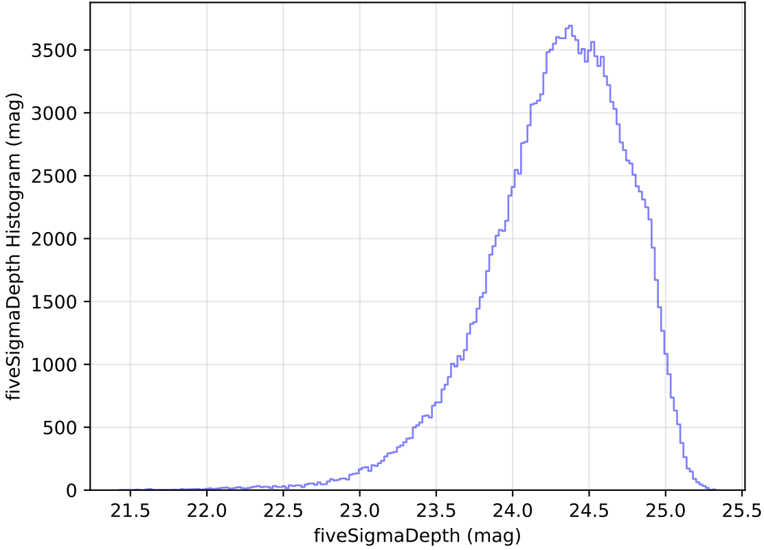
baseline_v3.2_10yrs WFD g band: fiveSigmaDepth Histogram
