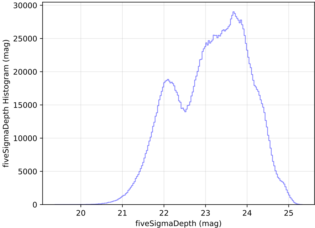
baseline_v3.2_10yrs WFD all bands: fiveSigmaDepth Histogram
