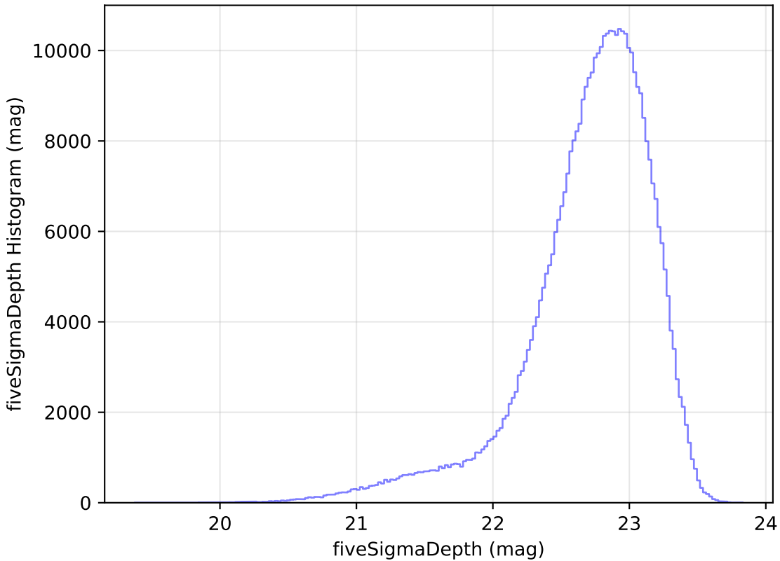
baseline_v3.2_10yrs All sky z band: fiveSigmaDepth Histogram
