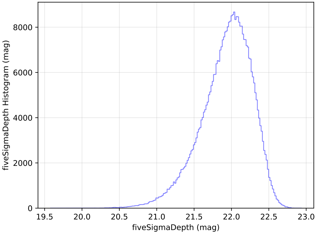
baseline_v3.2_10yrs All sky y band: fiveSigmaDepth Histogram
