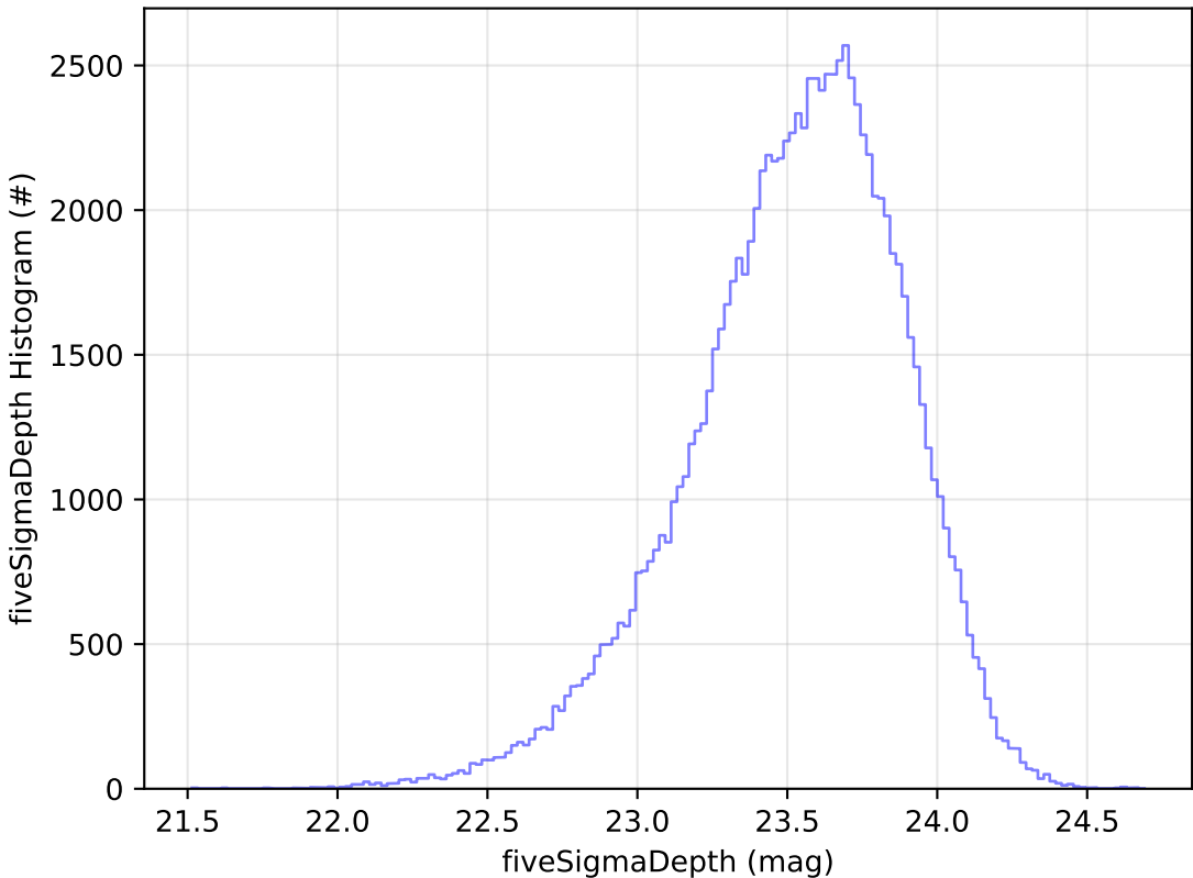
baseline_v3.2_10yrs All sky u band: fiveSigmaDepth Histogram
