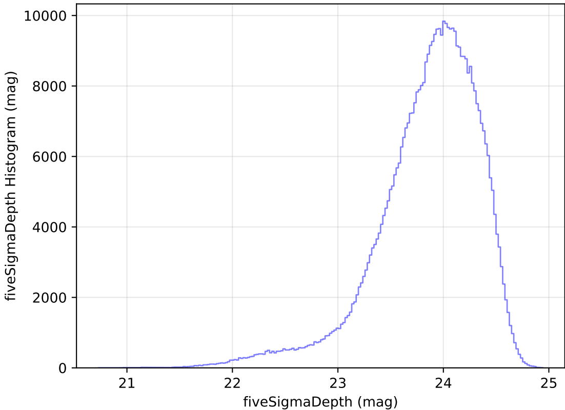
baseline_v3.2_10yrs All sky r band: fiveSigmaDepth Histogram
