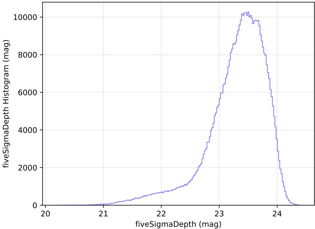
baseline_v3.2_10yrs All sky i band: fiveSigmaDepth Histogram
