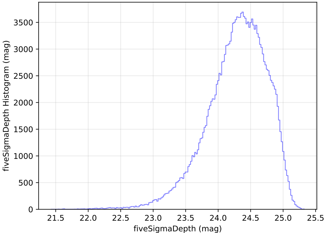
baseline_v3.2_10yrs All sky g band: fiveSigmaDepth Histogram
