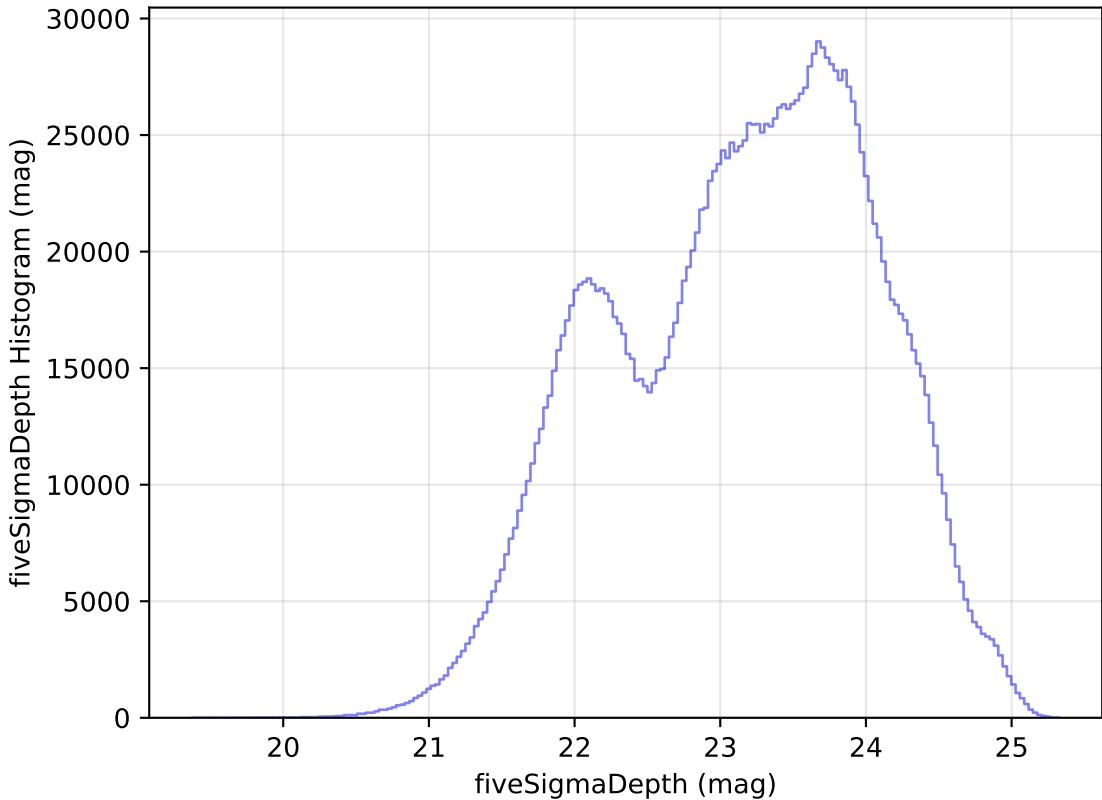
baseline_v3.2_10yrs All sky all bands: fiveSigmaDepth Histogram
