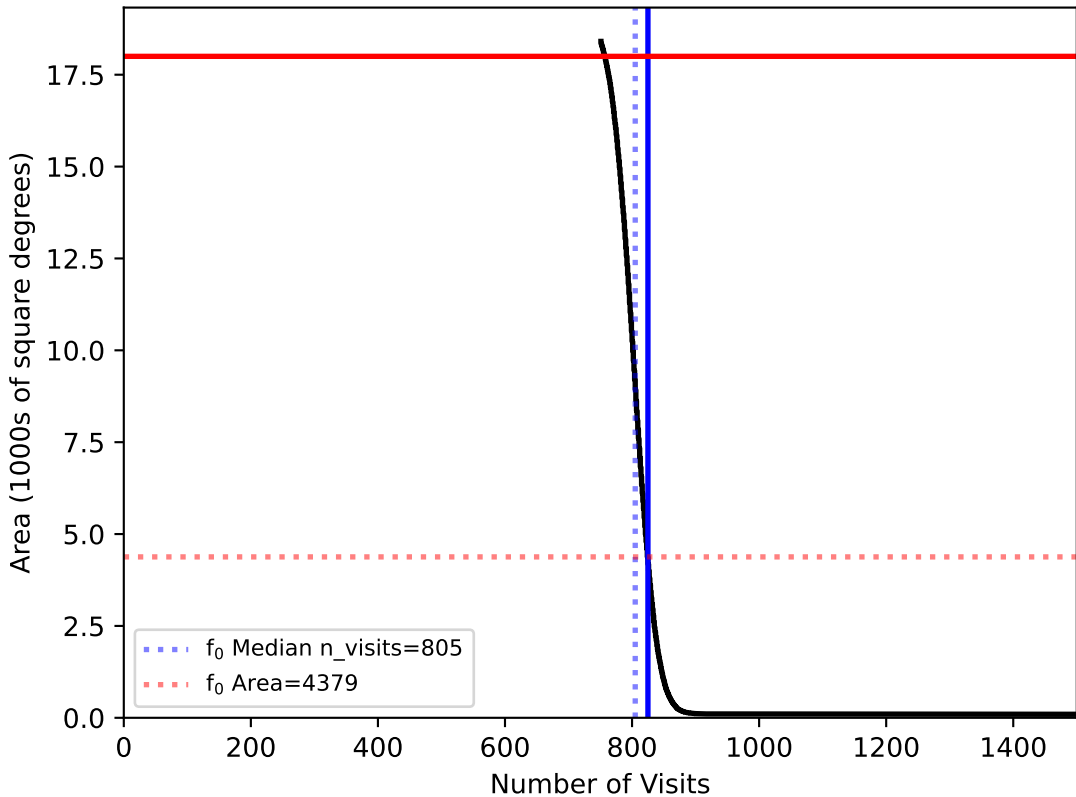
baseline_v3.2_10yrs WFD: f0
