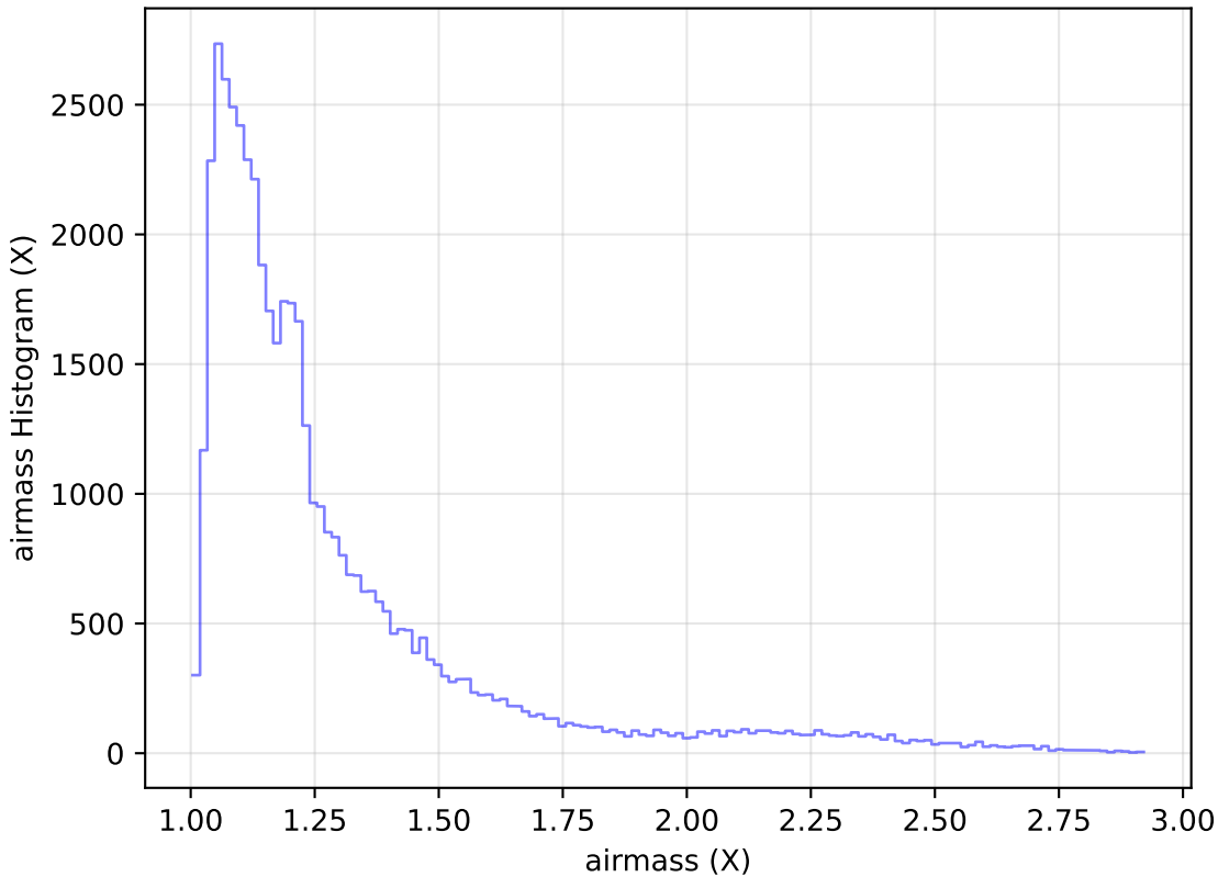
baseline_v3.2_10yrs Yr 1 z band: airmass Histogram
