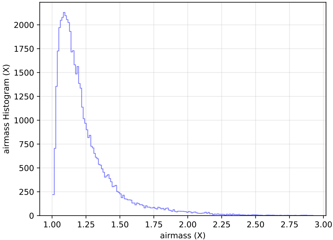
baseline_v3.2_10yrs Yr 1 y band: airmass Histogram
