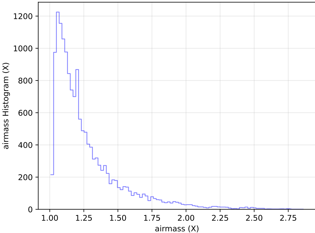
baseline_v3.2_10yrs Yr 1 u band: airmass Histogram
