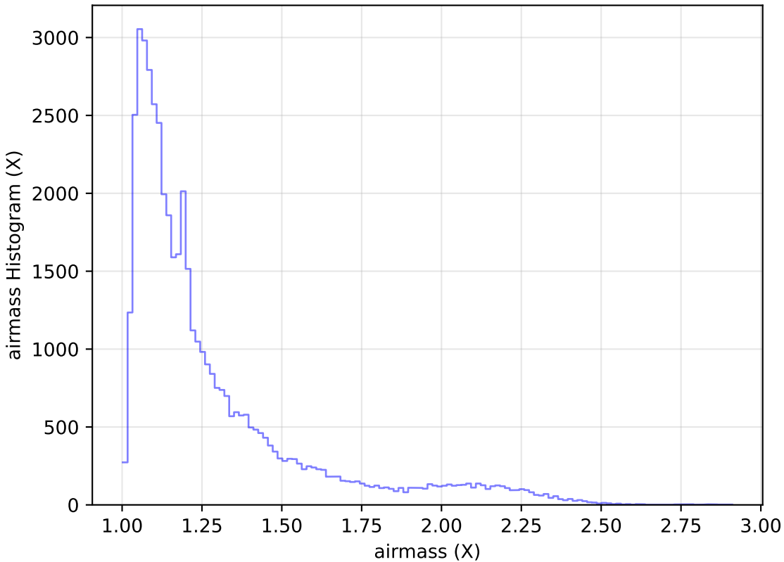
baseline_v3.2_10yrs Yr 1 r band: airmass Histogram
