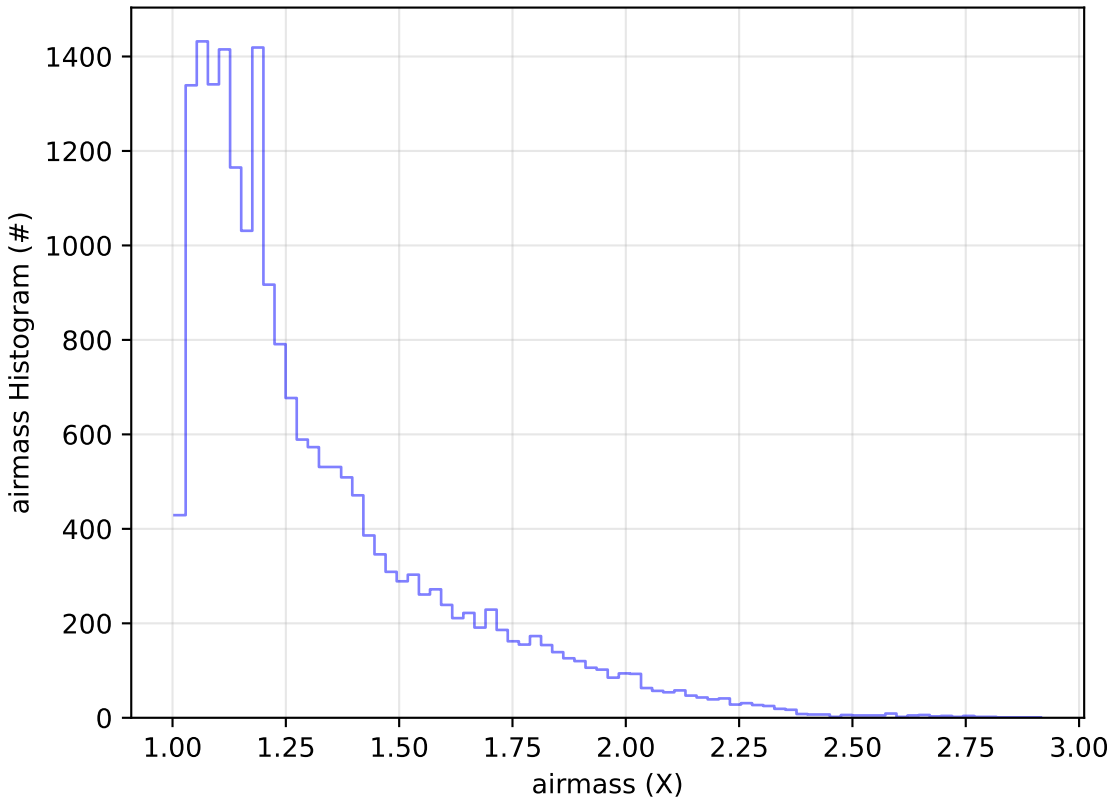
baseline_v3.2_10yrs Yr 1 g band: airmass Histogram
