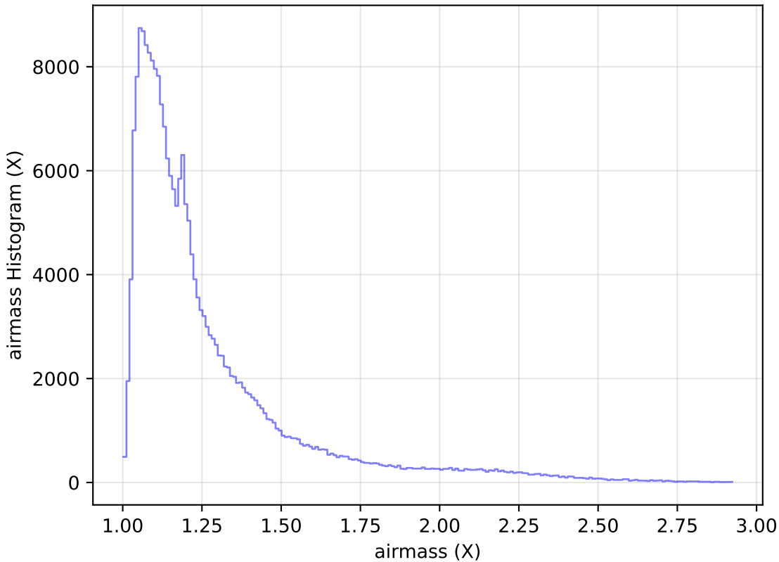
baseline_v3.2_10yrs Yr 1 all bands: airmass Histogram
