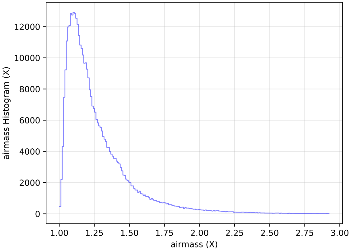
baseline_v3.2_10yrs WFD y band: airmass Histogram
