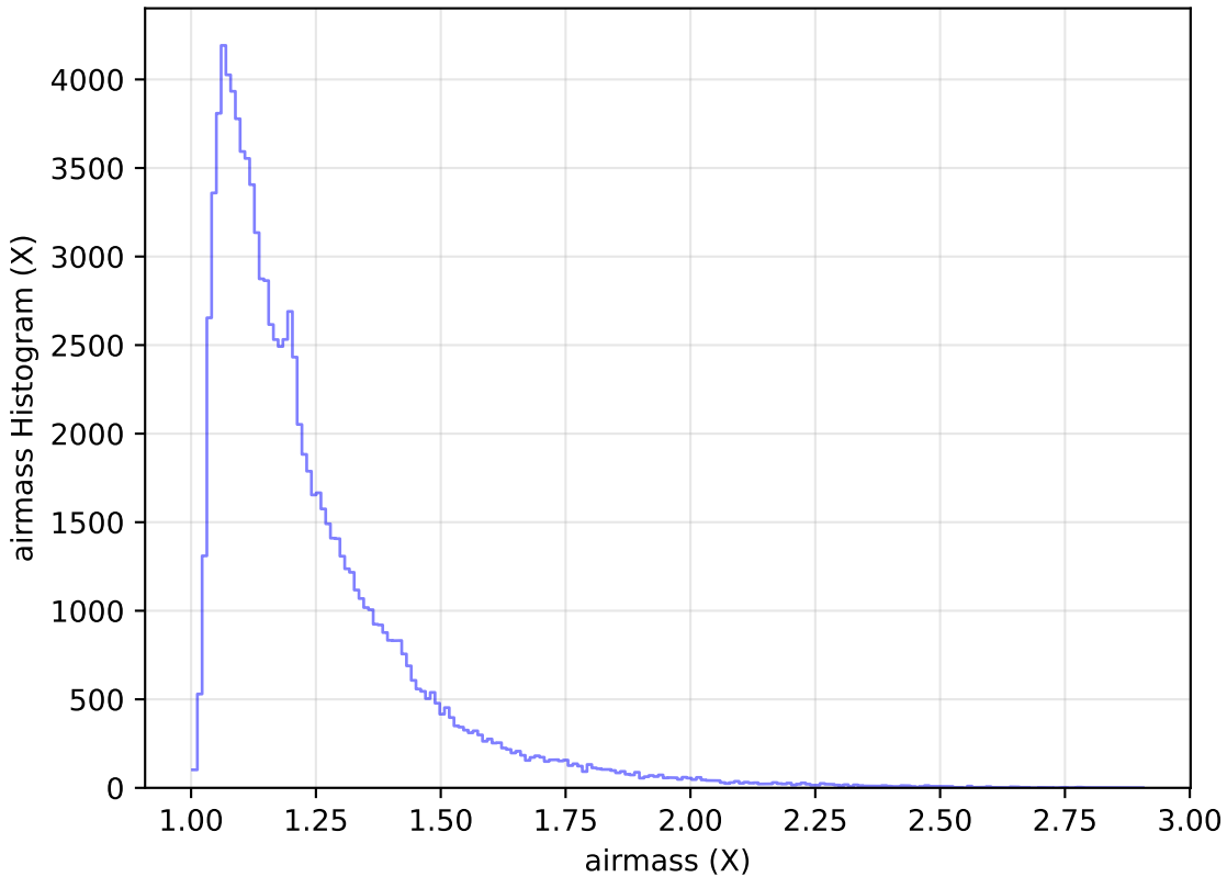
baseline_v3.2_10yrs WFD u band: airmass Histogram
