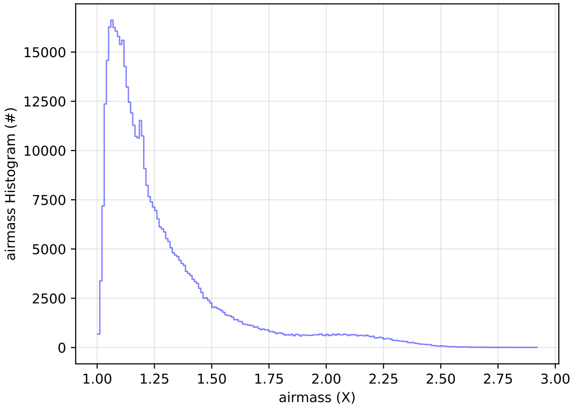
baseline_v3.2_10yrs WFD r band: airmass Histogram
