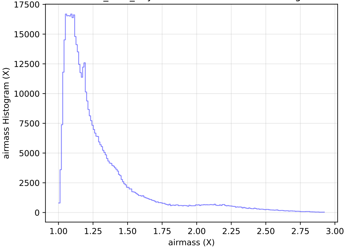
baseline_v3.2_10yrs WFD i band: airmass Histogram
