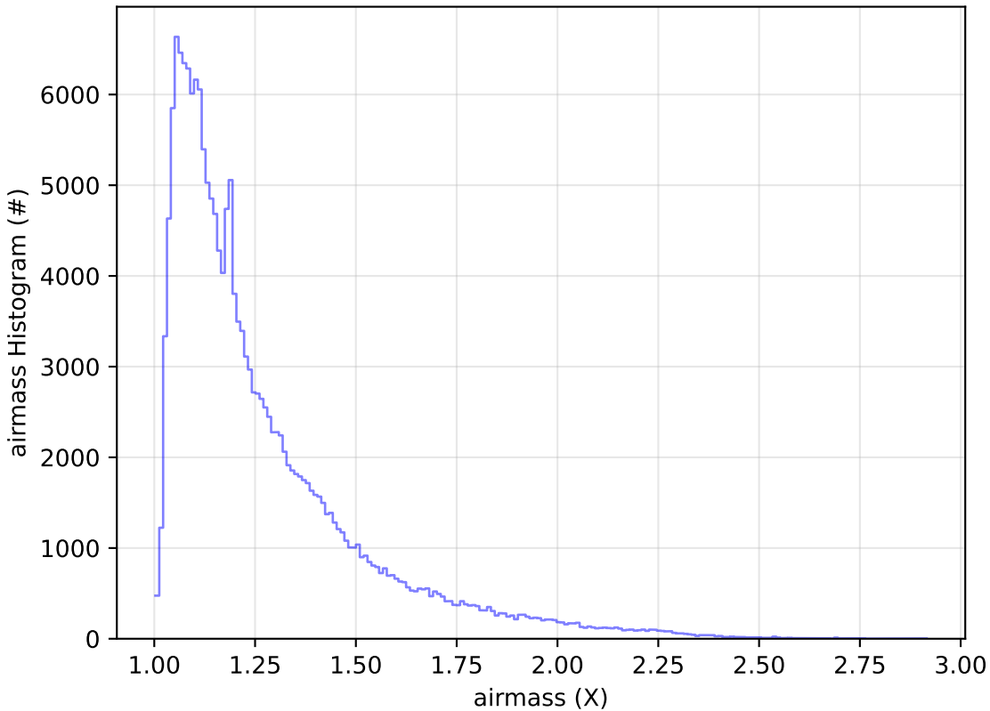
baseline_v3.2_10yrs WFD g band: airmass Histogram
