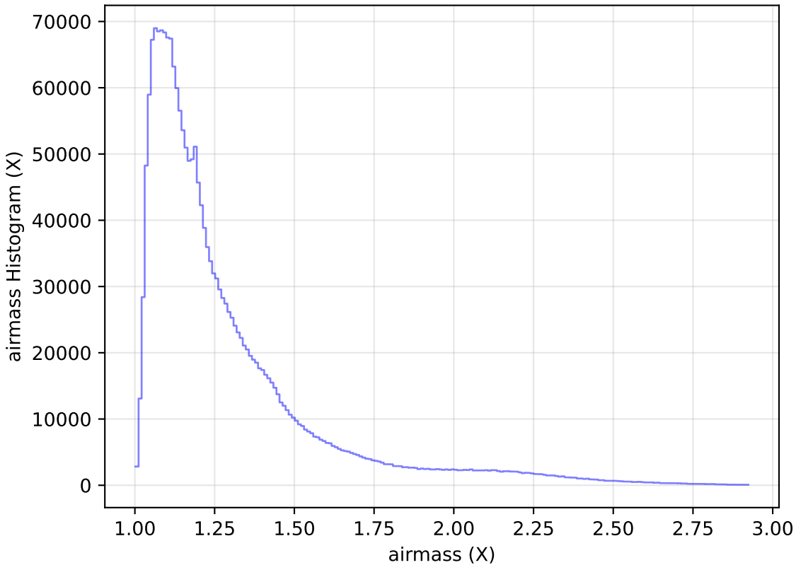
baseline_v3.2_10yrs WFD all bands: airmass Histogram
