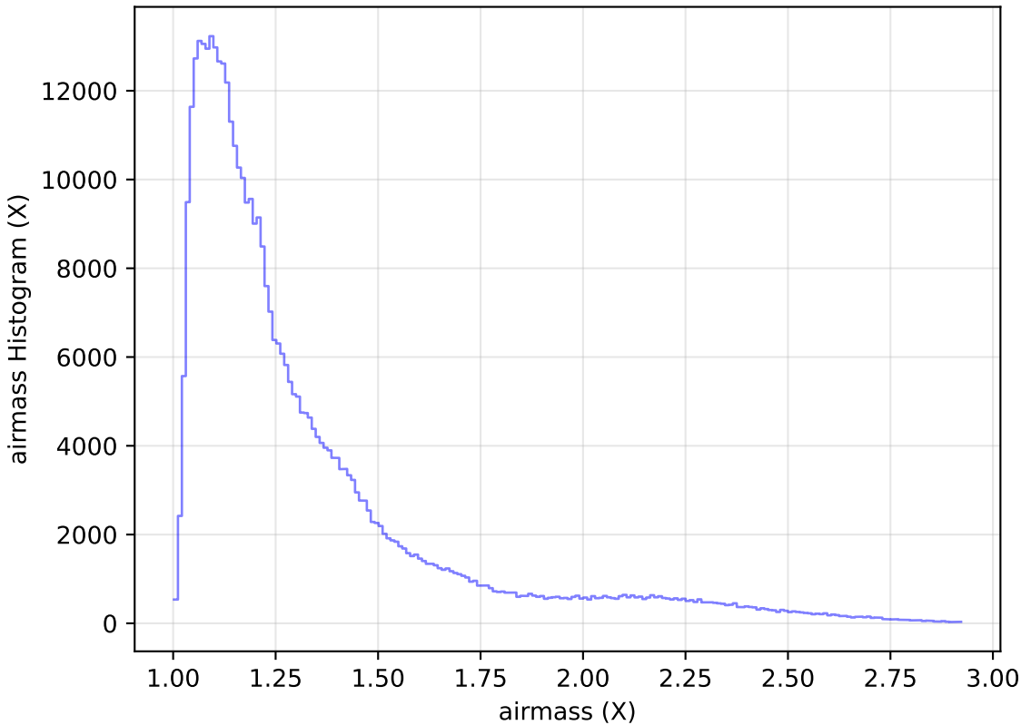
baseline_v3.2_10yrs All sky z band: airmass Histogram
