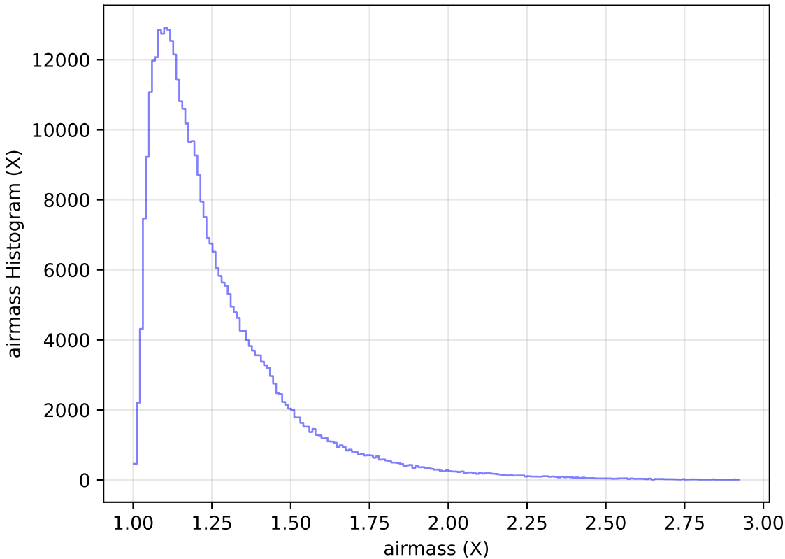
baseline_v3.2_10yrs All sky y band: airmass Histogram
