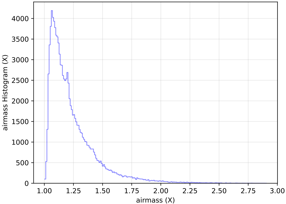
baseline_v3.2_10yrs All sky u band: airmass Histogram
