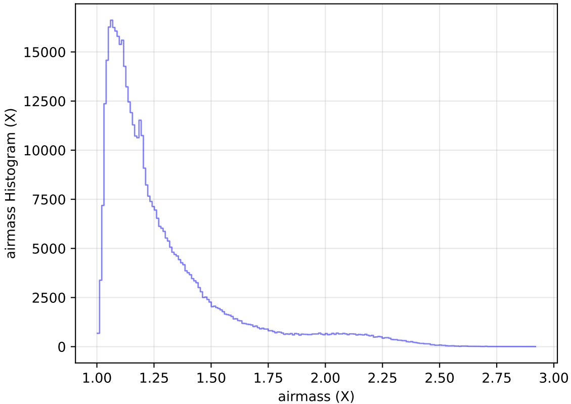
baseline_v3.2_10yrs All sky r band: airmass Histogram
