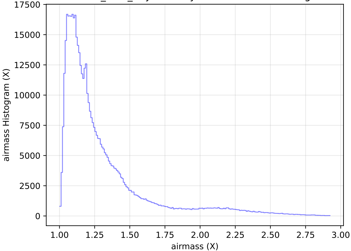
baseline_v3.2_10yrs All sky i band: airmass Histogram
