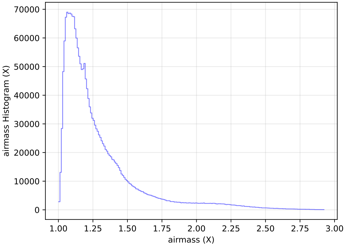
baseline_v3.2_10yrs All sky all bands: airmass Histogram
