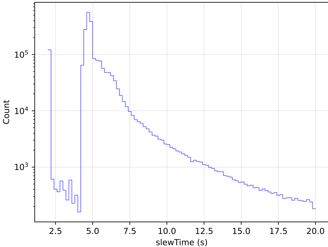
baseline_v3.2_10yrs All visits: Zoom Slew Time Histogram
