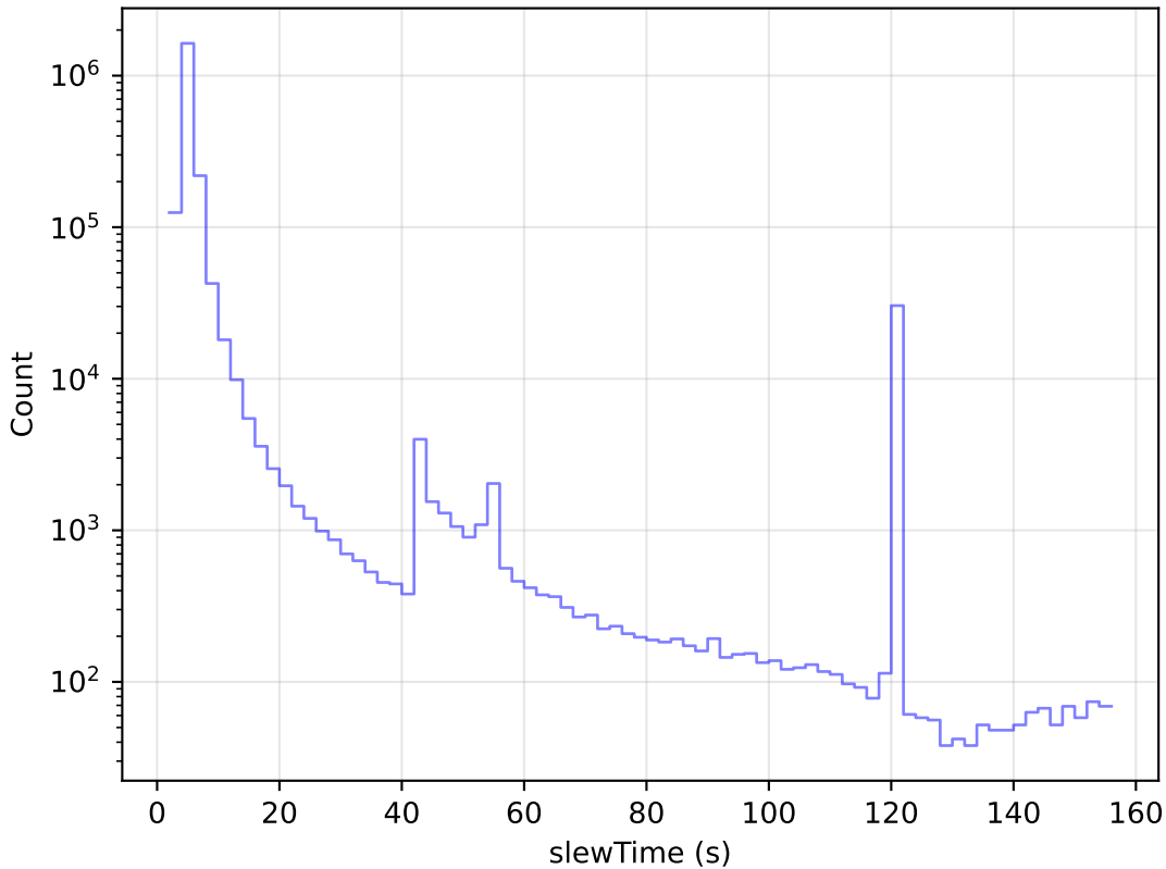
baseline_v3.2_10yrs All visits: Slew Time Histogram
