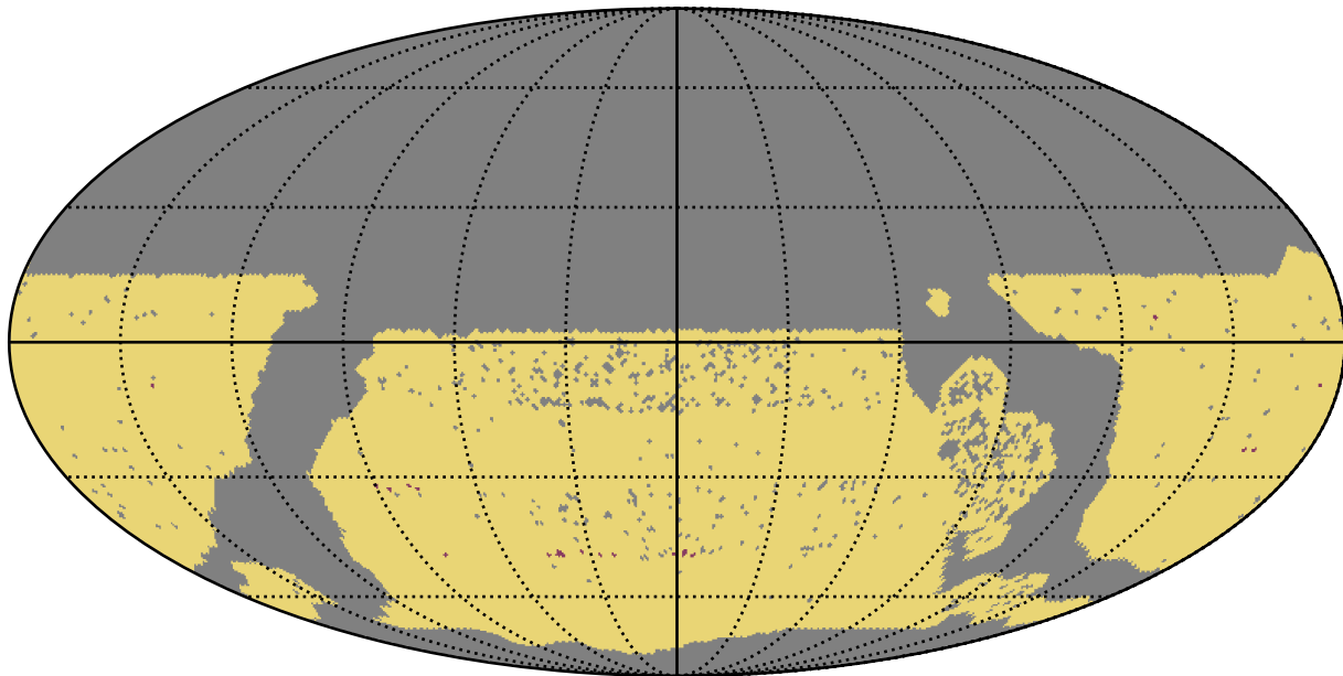
baseline_v3.2_10yrs WFD: RapidRevisits
