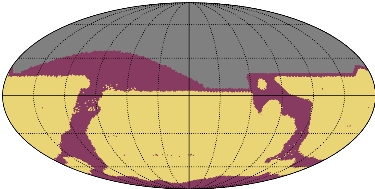
baseline_v3.2_10yrs All sky: RapidRevisits
