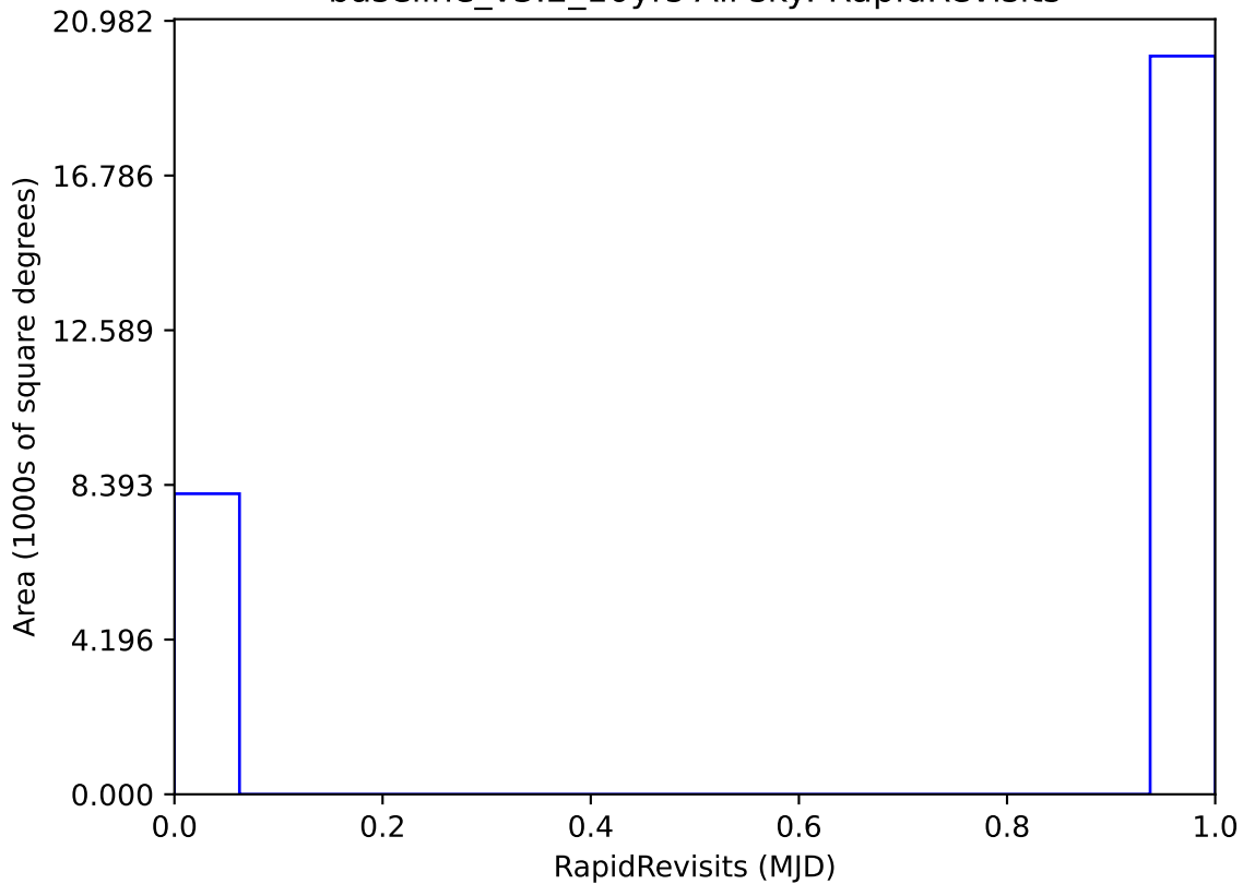
baseline_v3.2_10yrs All sky: RapidRevisits
