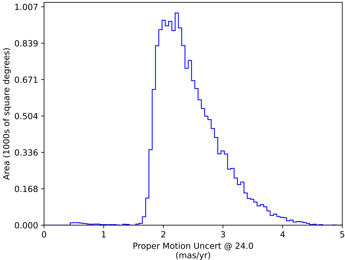
baseline_v3.2_10yrs WFD: Proper Motion Uncert @ 24.0
