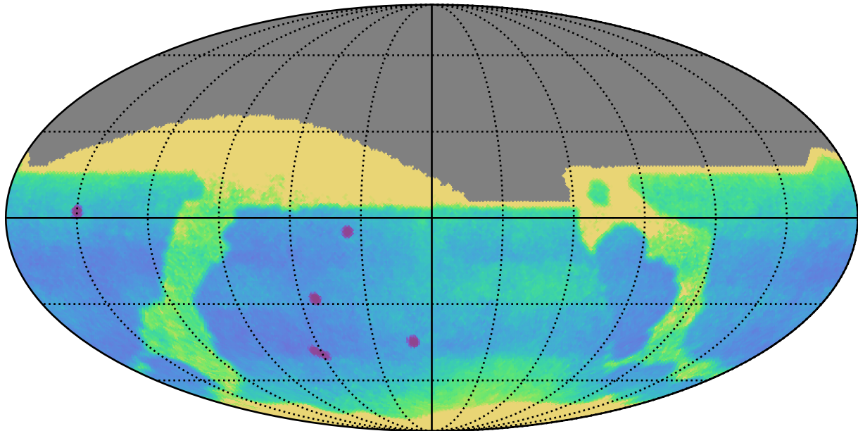
baseline_v3.2_10yrs All sky: Proper Motion Uncert @ 24.0
