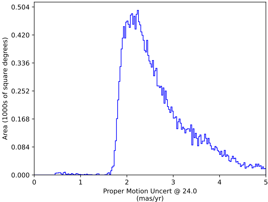
baseline_v3.2_10yrs All sky: Proper Motion Uncert @ 24.0
